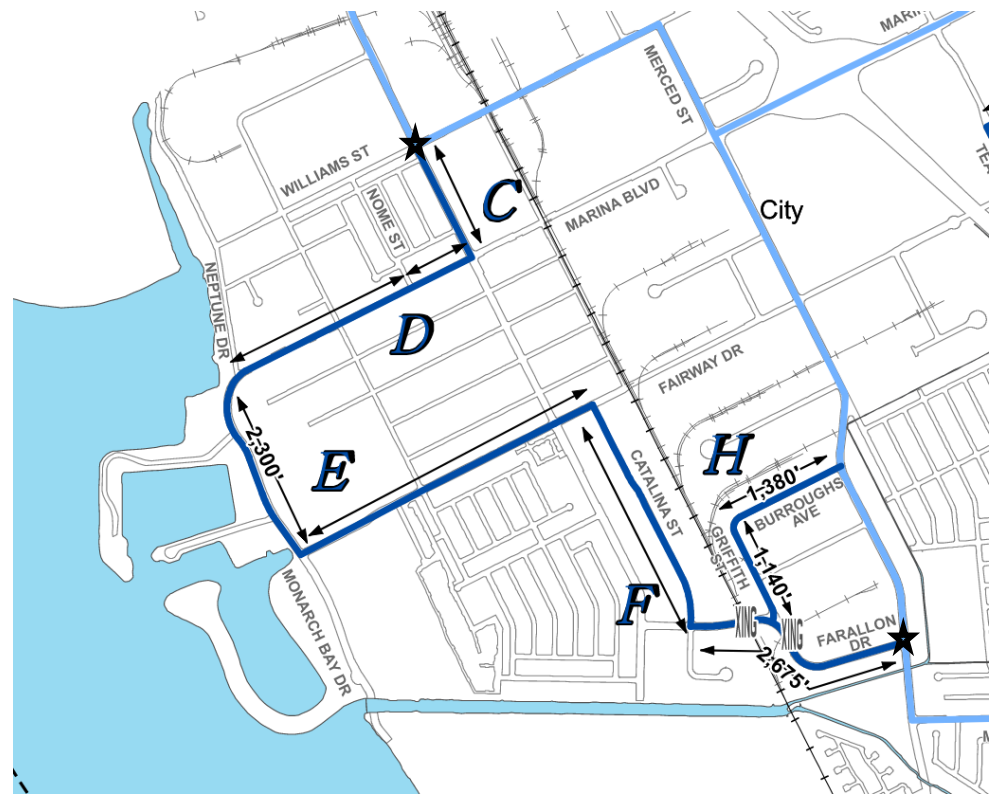
Sections C,D,E,F encompasses where fiber optic cable will be installed.
