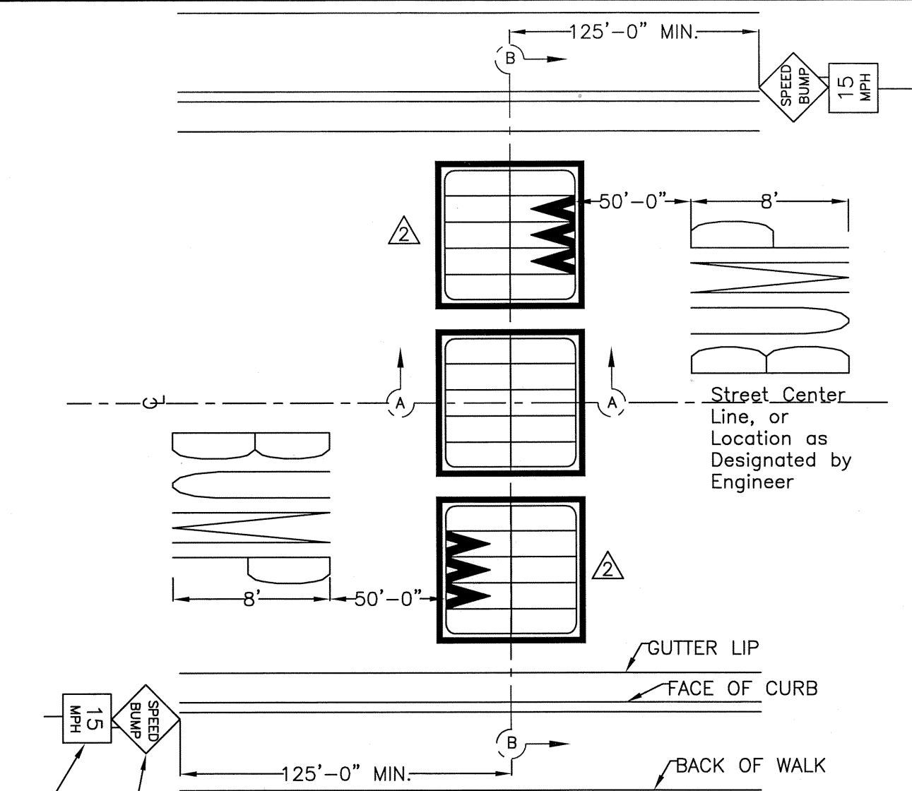
PLAN
