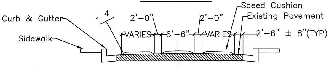
SECTION B-B
